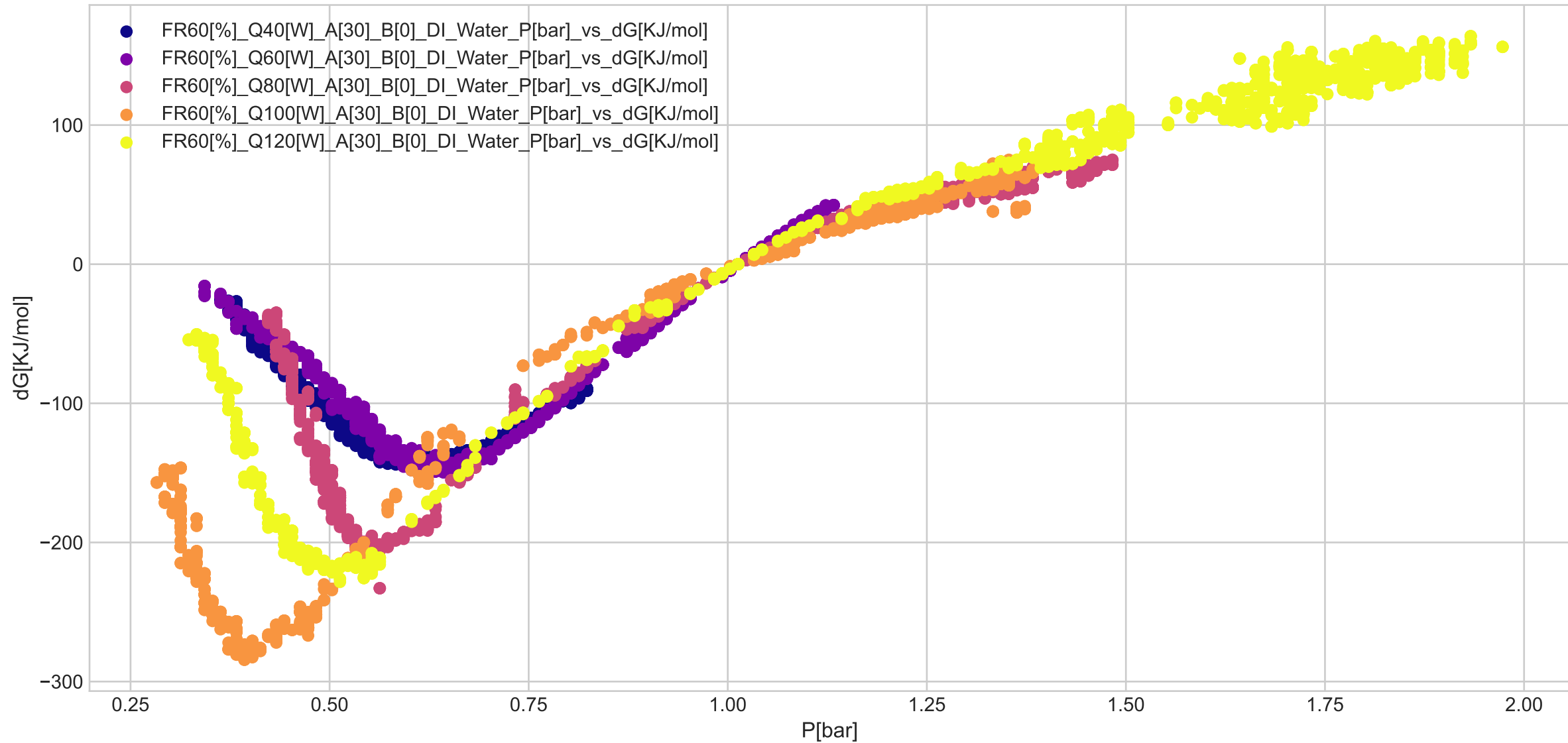
FR [60]% - Q [ 40 60 80 100 120]W - alpha [30] - beta [0] - DI_Water
